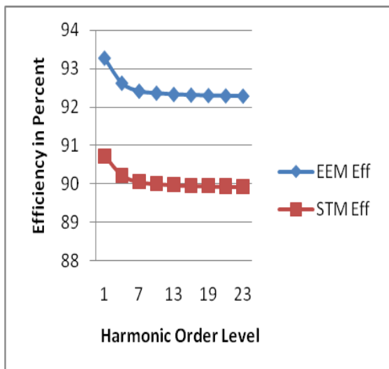
Figure 7: Efficiencies for 25 HP Motors vs. Harmonic Order
