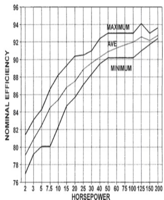
Figure 1: Nominal efficiency range of standard open NEMA design B 1800-rpm polyphase induction motors.
