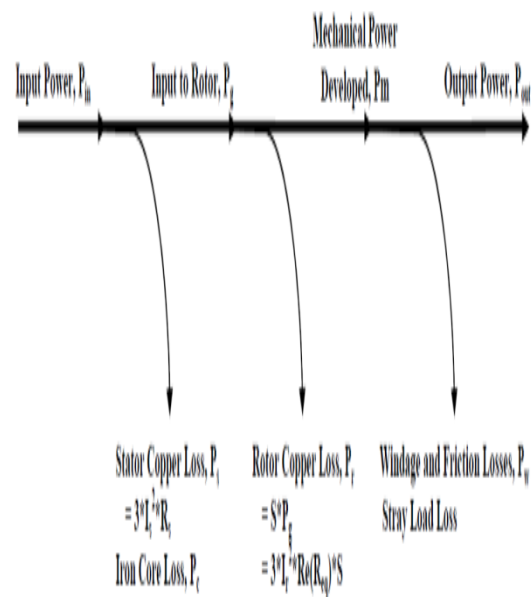
Figure 3: Power Flow in an Induction Motor
