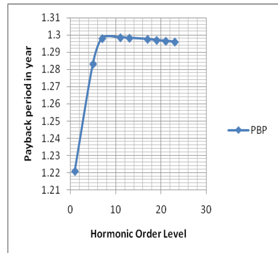
Figure 9: Payback Time for 25 HP Motors vs. Harmonic
