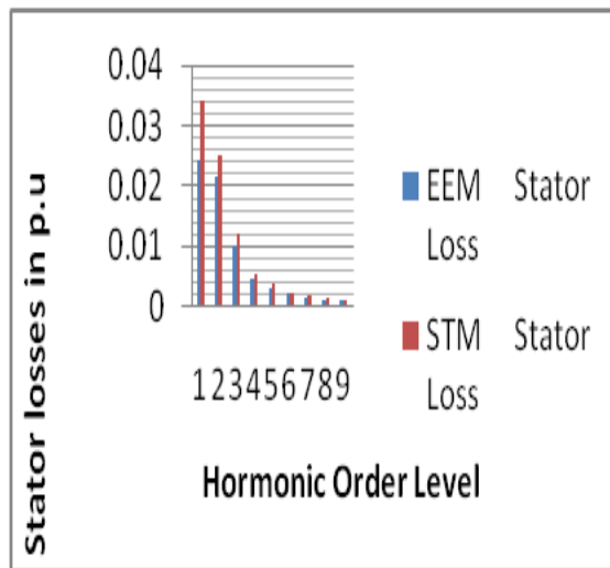
Figure 6: Stator Losses for 25 HP Motors vs. Harmonic Order
