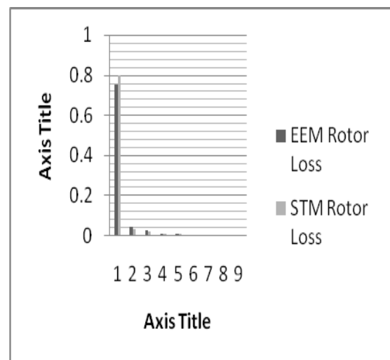
Figure 5: Rotor Losses for 25HP Motors vs. Harmonic Order
