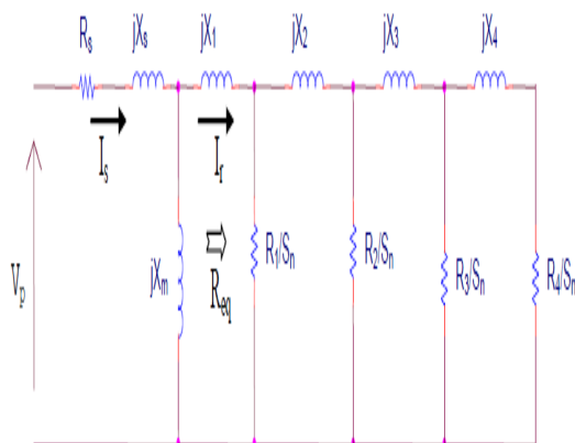
Figure 2: The Skin Effect Impedance Model
