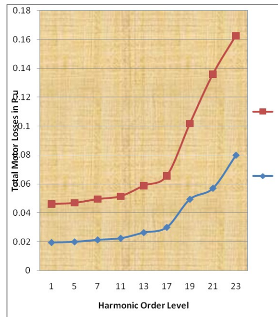
Figure. 4: Cumulative Total Losses for 25HP Motors
