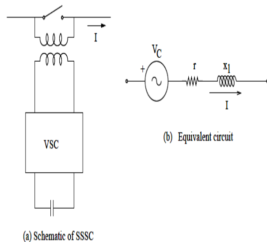
Figure 1. Schematic of SSSC. [2]
