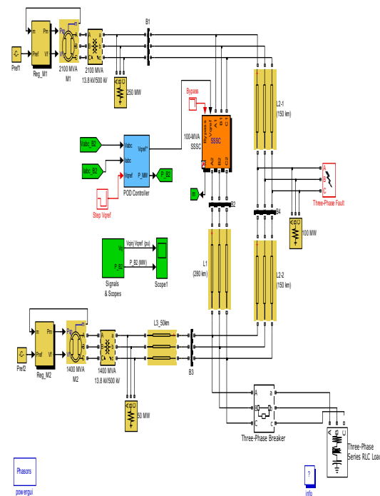
Figure 2: Simulink diagram representation of proposed work.
